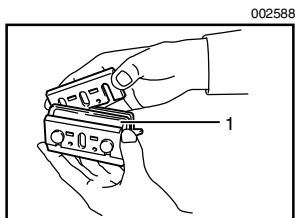
1. Sharpening holder
