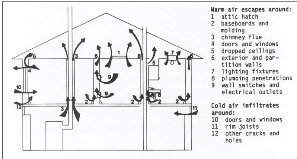
Figure 3: Common Air Leakage Sites
