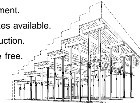
Typical Shoring Post Applicaton
