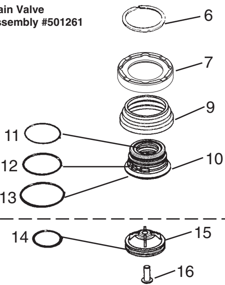
Piston Assembly #501268
