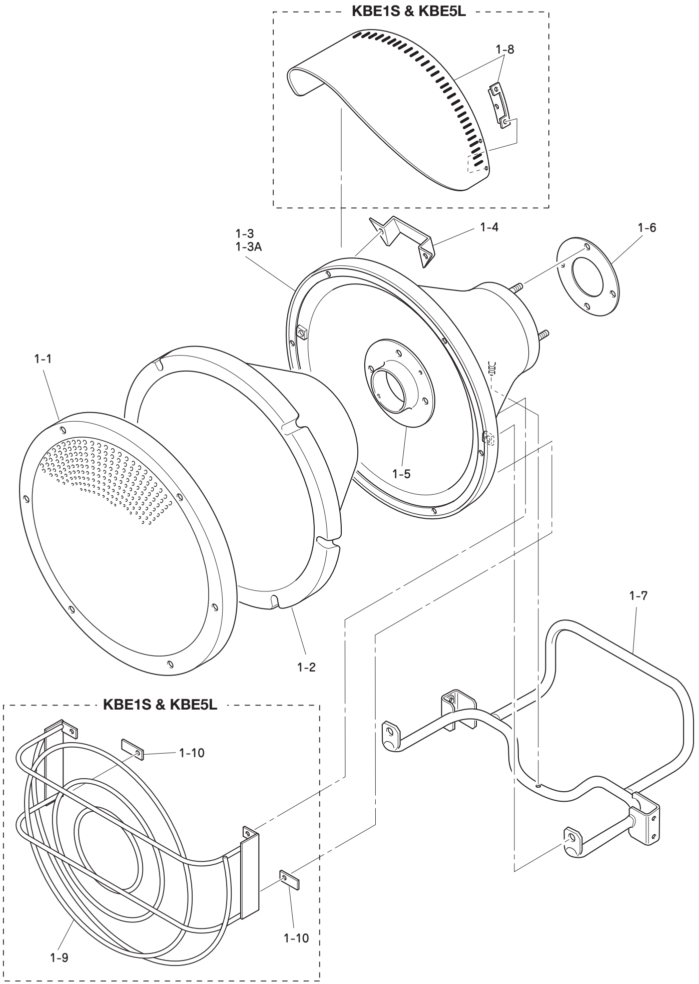
VAL6 KBE1S/5S/5L Radiation Section_ Revised 2011
