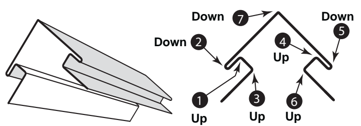
7. Counter Flashing
