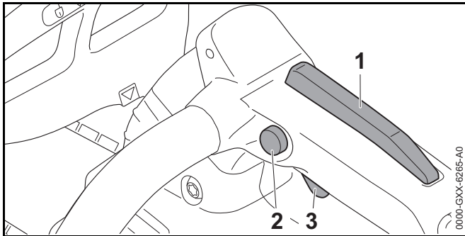
Ergo-Lever (1), Trigger Switch Lockout (2) and Trigger Switch (3)
