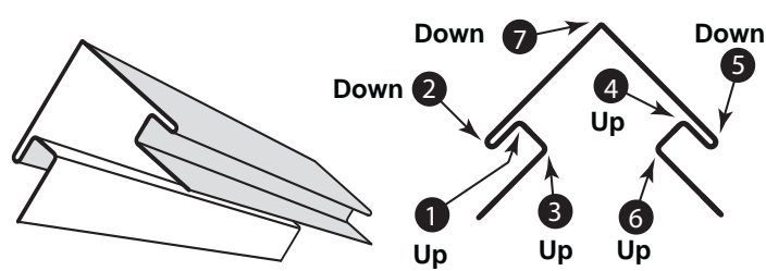
7. Counter Flashing
