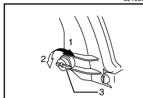
1. Release 2. Lock 3. Lock lever
