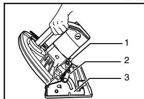
1. Clamp screw 2. Lever 3. Bevel scale plate
